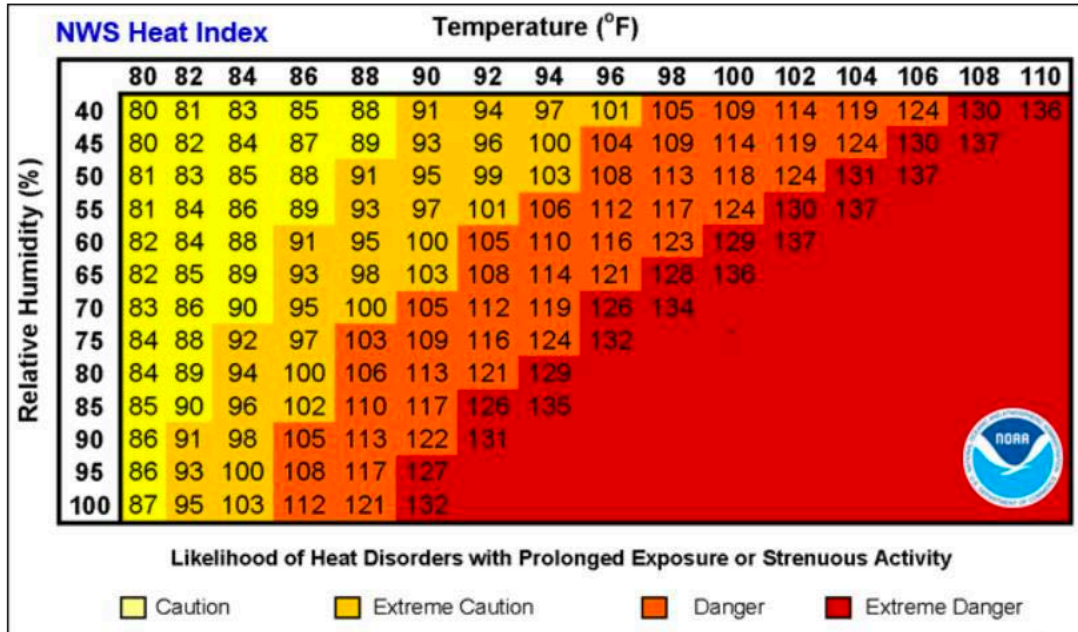
Figure 28: Heat Index
