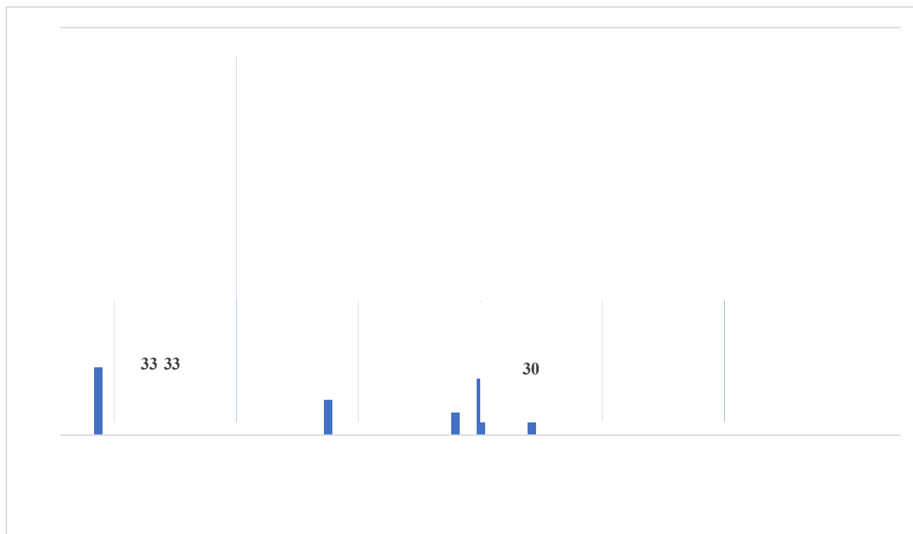
Figure 45: Flood/Flash Flood Events by County, 1997-2022
