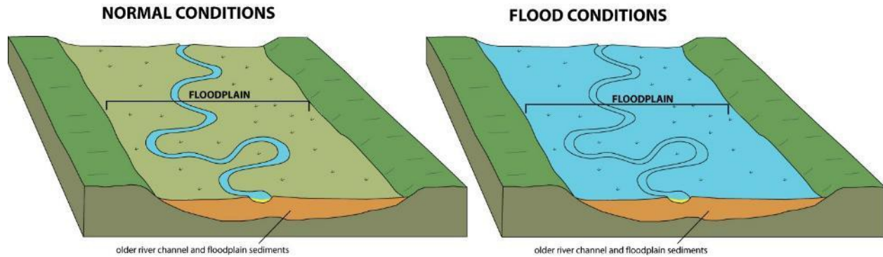
Figure 34: Flood Definition
