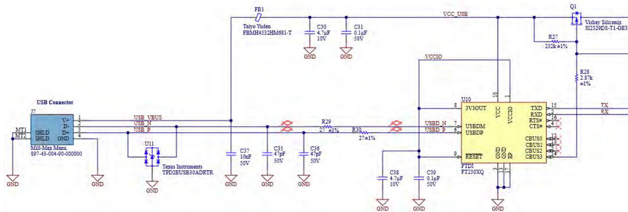
Figure 1: Schematic of USB Interface
